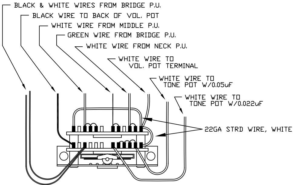
SWITCH WIRING DETAIL
